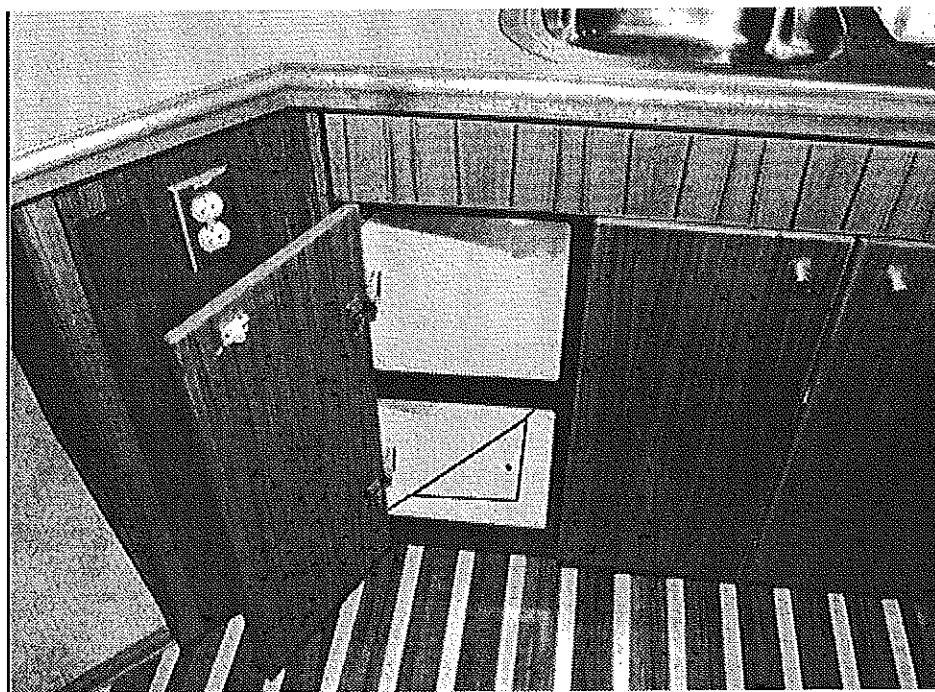
Port Fuel Pick-up Tube Access
