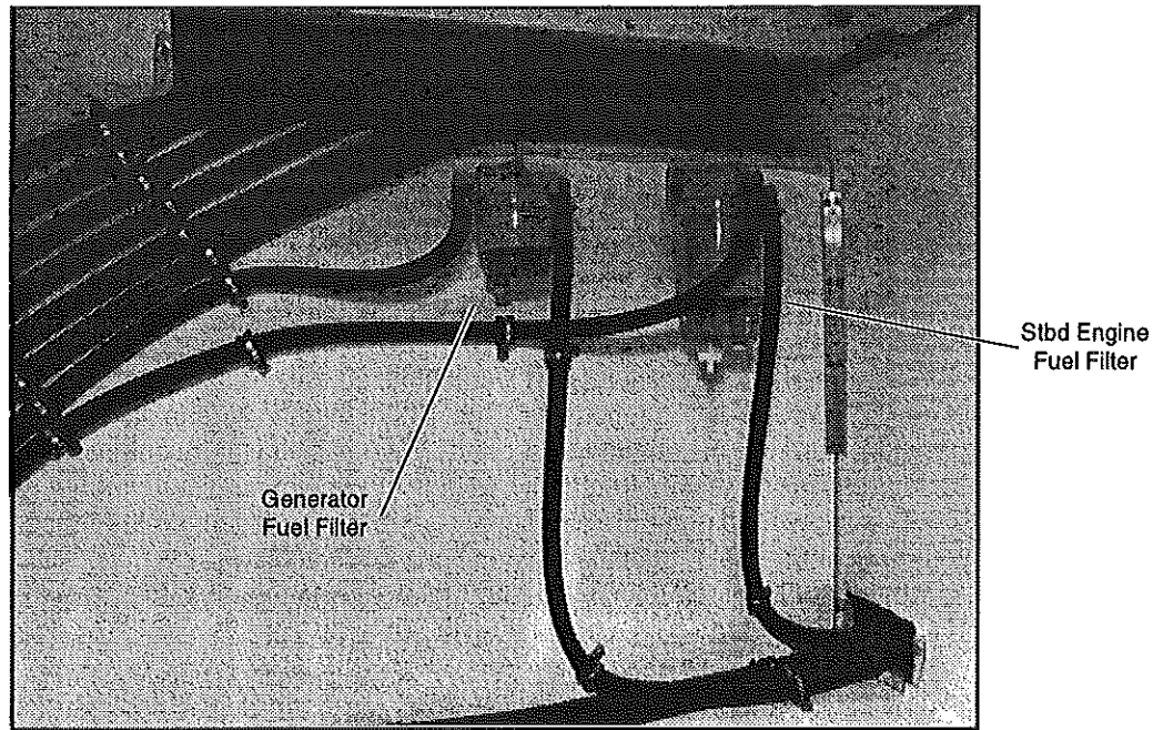
Starboard Fuel Filter Layout
